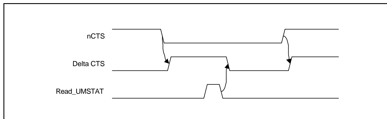
Figure 11-8. nCTS and Delta CTS Timing Diagram
