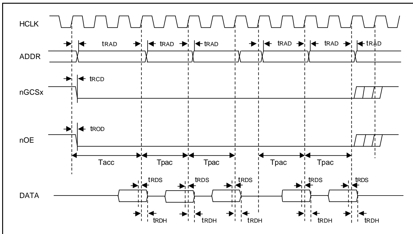
Figure 27-19. Masked-ROM Consecutive READ Timing Diagram ( T_{acs}=0 , T_{cos}=0 , T_{acc}=3 , T_{pac}=2 , PMC=01/10/11 )
