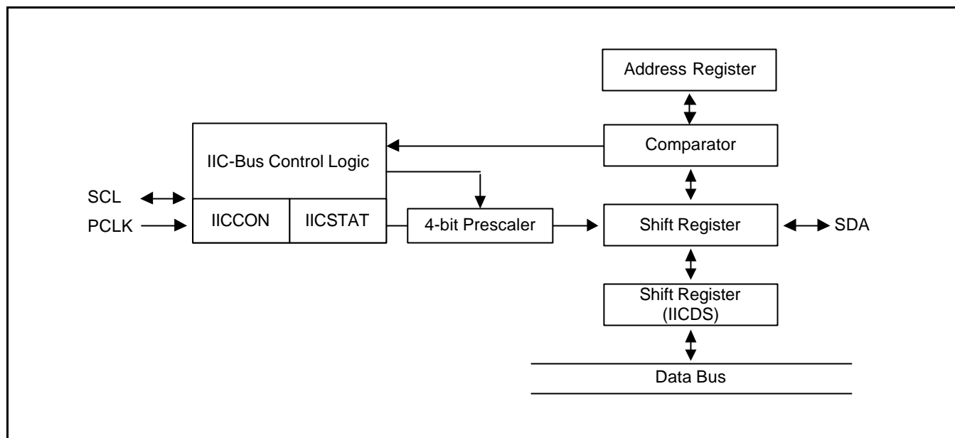
Figure 20-1. IIC-Bus Block Diagram
