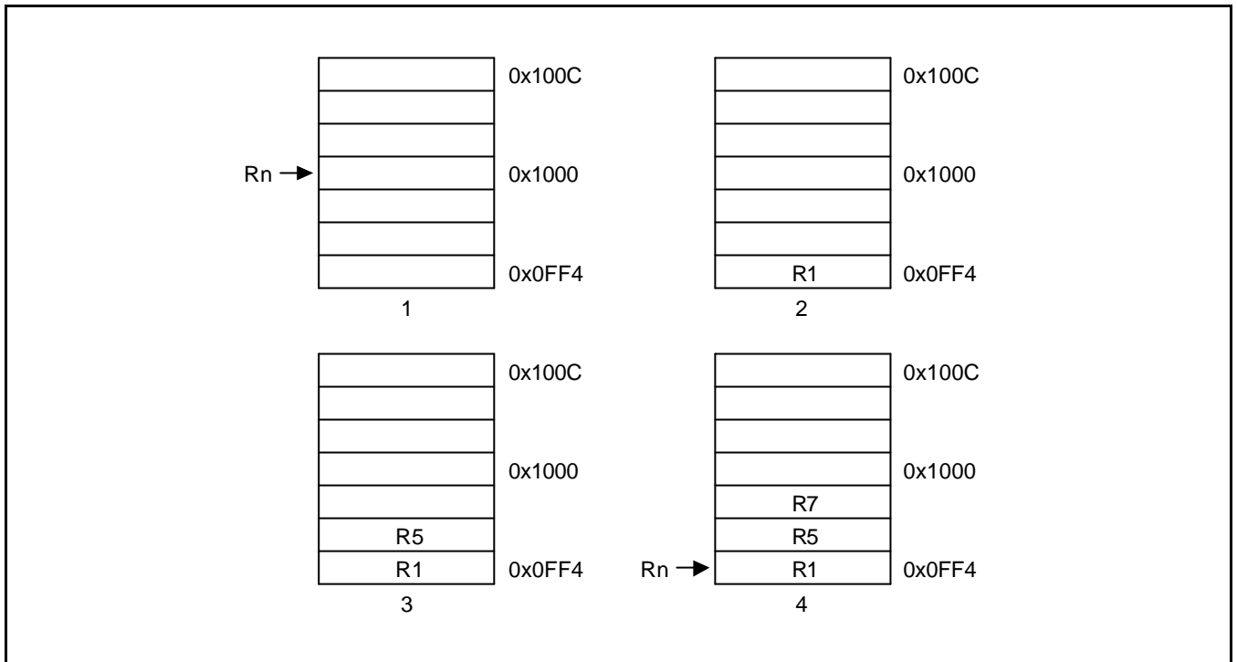
Figure 3-22. Pre-Decrement Addressing
