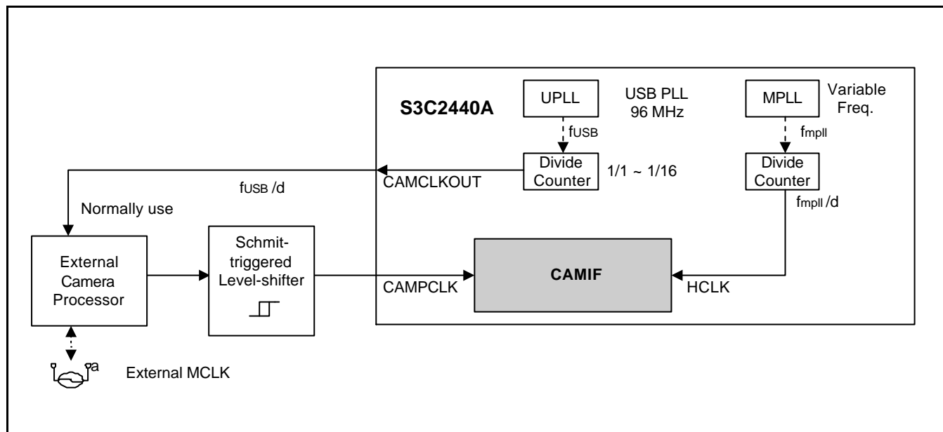
Figure 23-5. CAMIF Clock Generation
