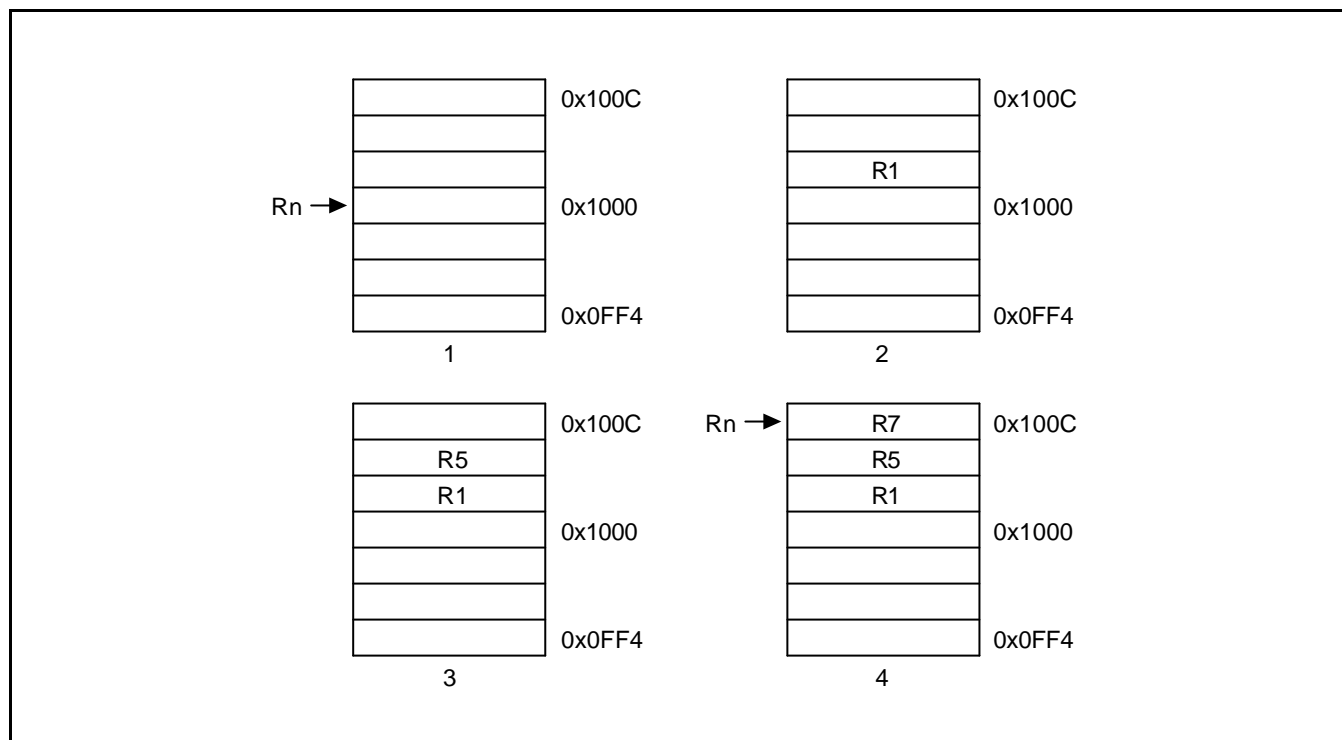
Figure 3-20. Pre-Increment Addressing
