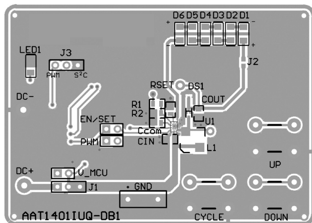
Figure 7: AAT1401 Evaluation Board Top Side Layout.
