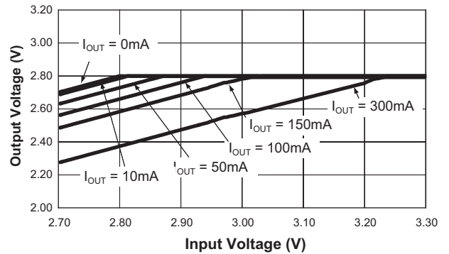
LDO Dropout Characteristics (EN = GND; ENLDO = V IN )
