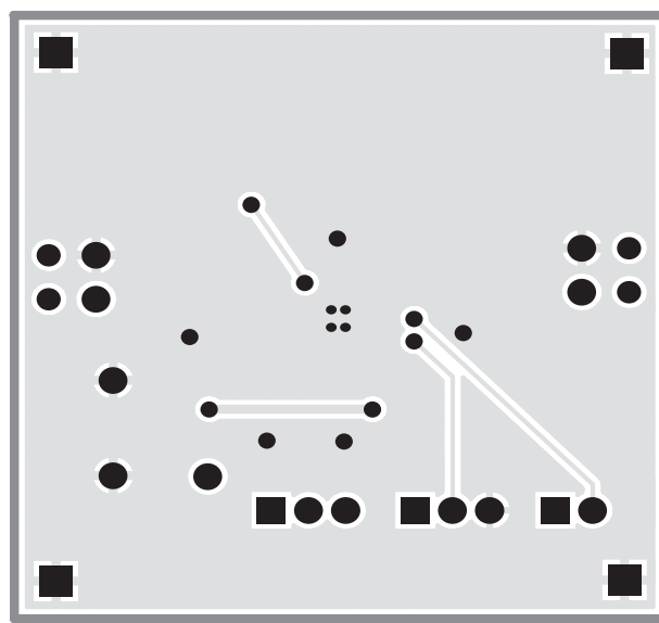
Figure 7: AAT2556 Evaluation Board Bottom Side Layout.
