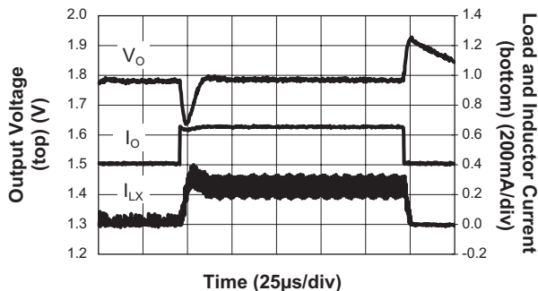
Load Transient Response (10mA to 250mA; V_{IN} = 3.6V ; V_{OUT} = 1.8V ; C_{OUT} = 4.7\mu F )
