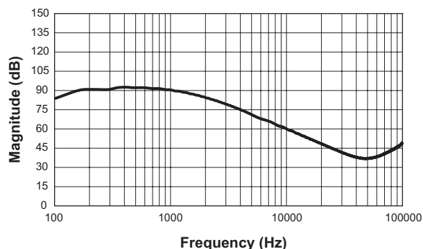
LDO Power Supply Rejection Ratio, PSRR ( I_{OUT3} = 10mA , BW = 100~100KHz)
