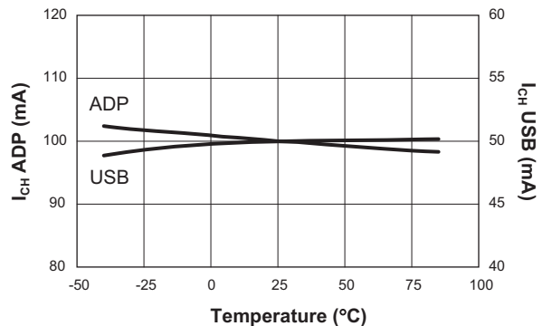
Preconditioning Charge Current vs. Temperature ( R_{SETADP} = 8.06k\Omega ; R_{SETUSB} = 8.06k\Omega )
