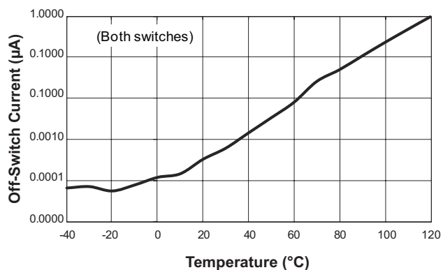
Off-Switch Current vs. temperature
