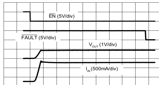
Start Into 1\Omega Load
