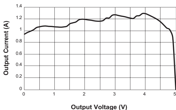
Current Limit
