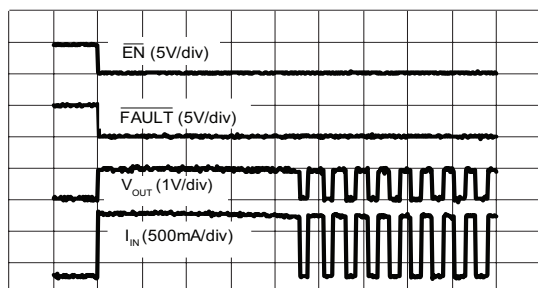
Thermal Shutdown Response
