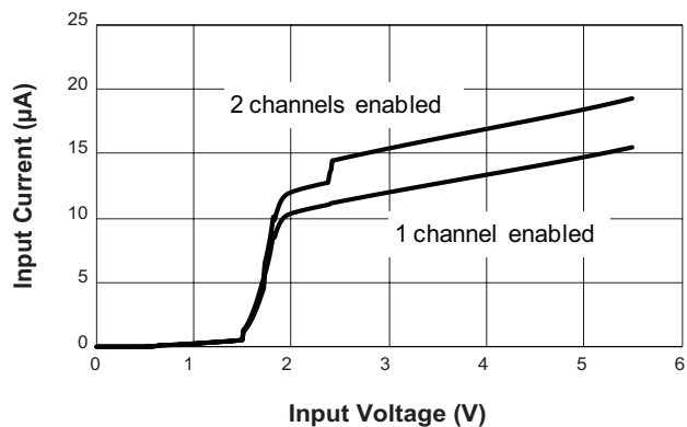
Quiescent Current
