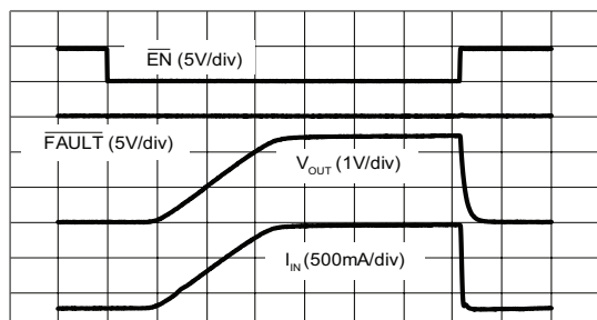
Turn On/Off Response with 10\Omega , 1\mu F Load
