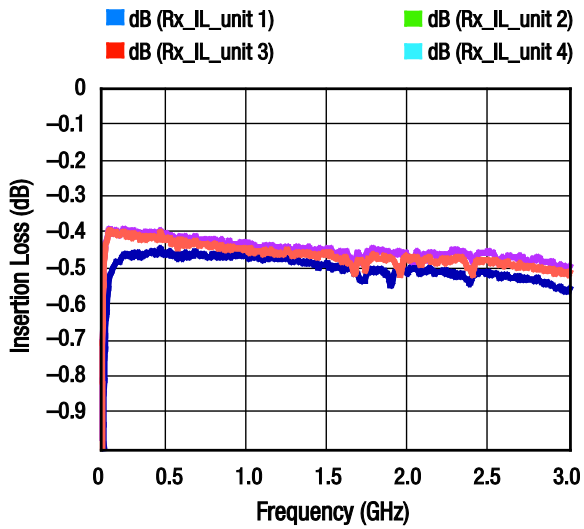
Figure 9. RFC to RF2 Insertion Loss
