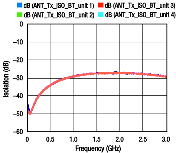
Figure 19. RF3 to RF1 Isolation
