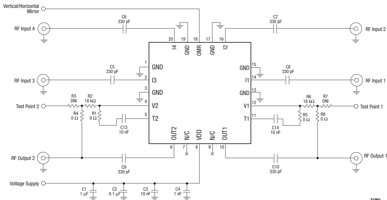
Figure 11. SKY13327-365LF Evaluation Board Schematic
