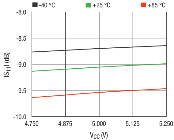
|S_{11}| vs. V_{CC} Across Temperature
