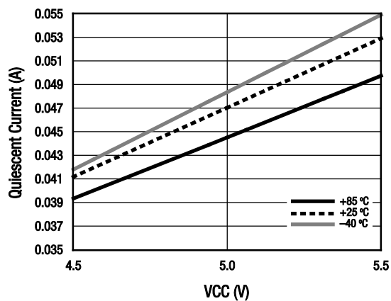
Figure 32. Quiescent Current vs VCC Over Temperature
