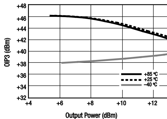
Figure 24. OIP3 vs Output Power Over Temperature
