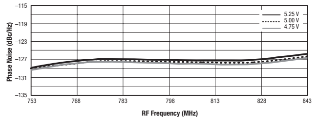
Figure 19. Phase Noise @ 200 kHz Offset vs Frequency and Supply Voltage
