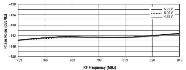
Figure 21. Phase Noise @ 400 kHz Offset vs Frequency and Supply Voltage
