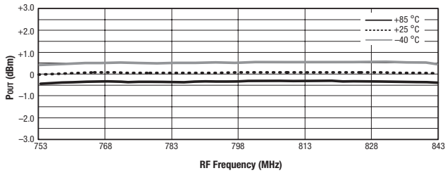
Figure 10. Output Power vs Frequency and Temperature
