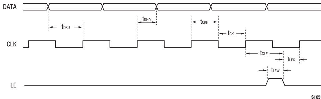
Figure 3. SKY73112-11 Serial Data Input Timing Diagram (MSB First)
