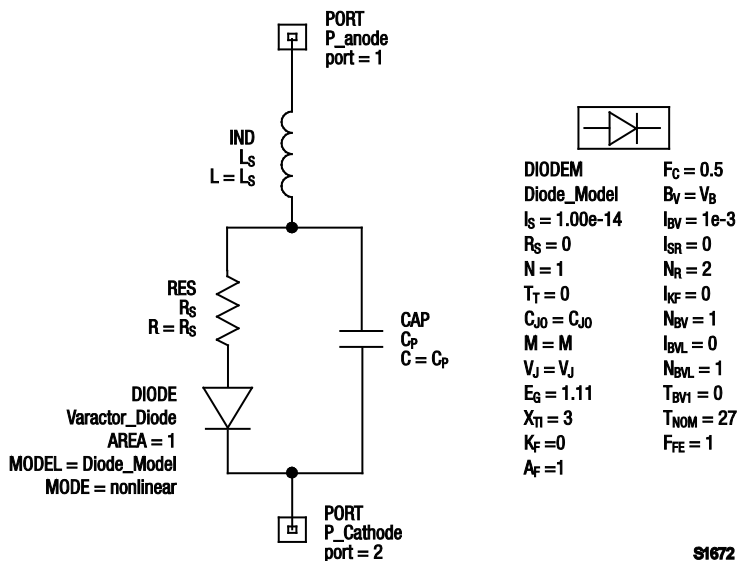
Figure 3. SPICE Model
