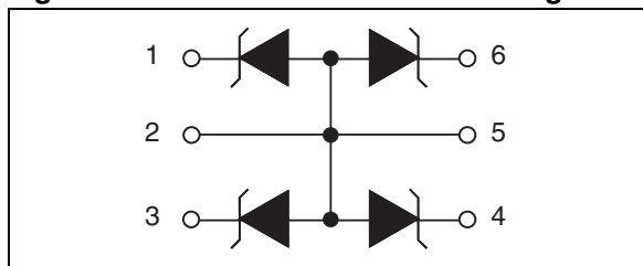
Figure 2. ESDAxxSC6 functional diagram
