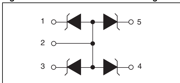
Figure 1. ESDAxxSC5 functional diagram
