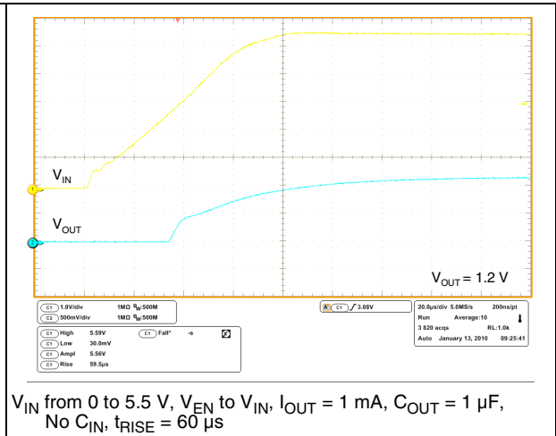
Figure 20. Startup transient
