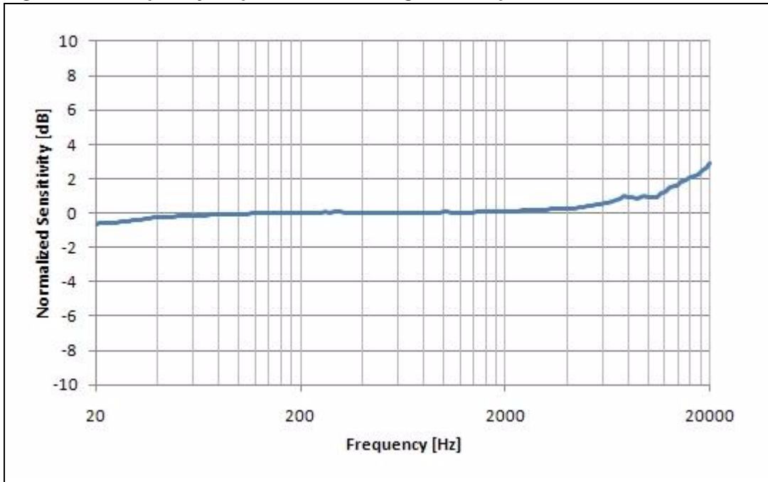
Figure 3. Frequency response mask for digital microphone
