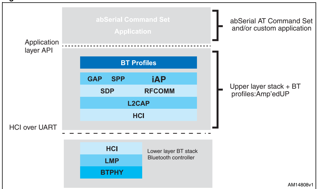
Figure 1. FW architecture
