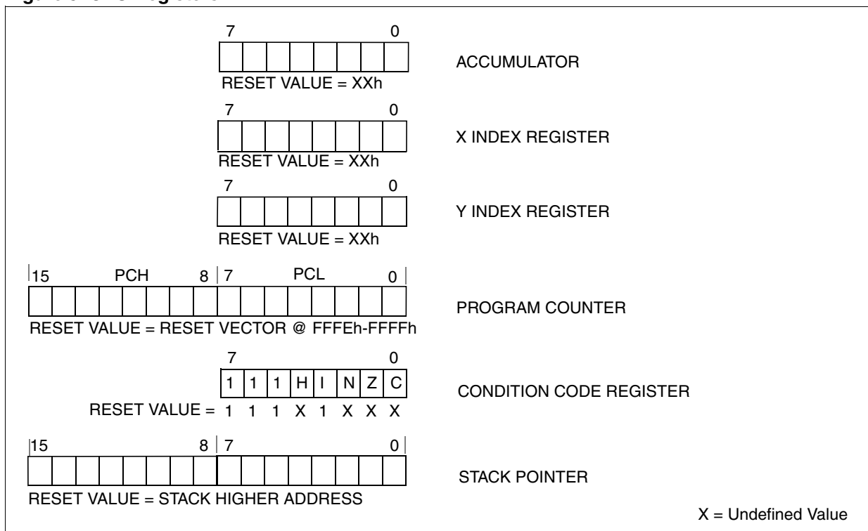
Figure 5. CPU Registers
