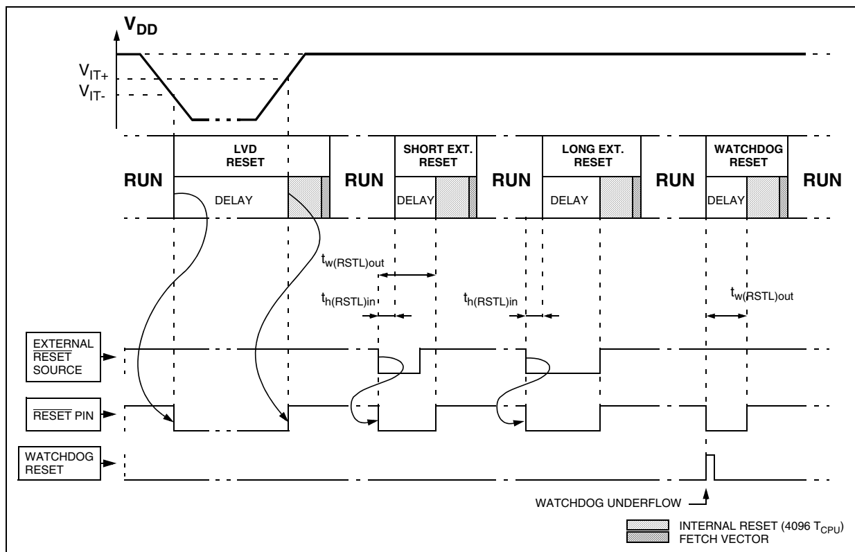
Figure 11. RESET Sequences
