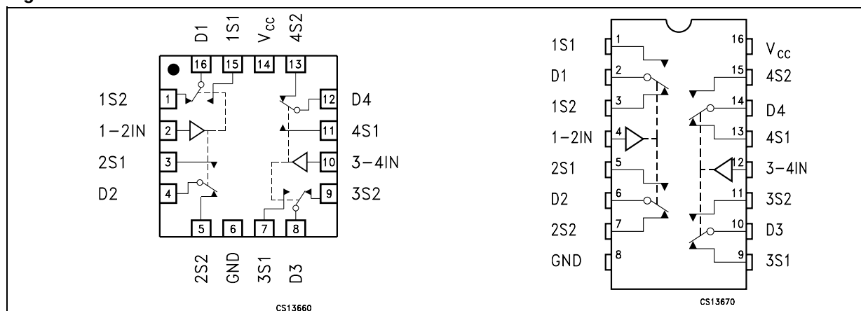
Figure 1: Pin Connection
