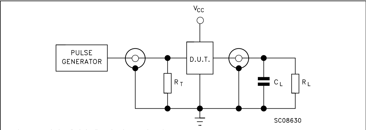
Figure 8: Test Circuit
