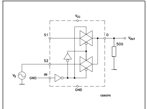
Figure 4: Schematic Bandwidth
