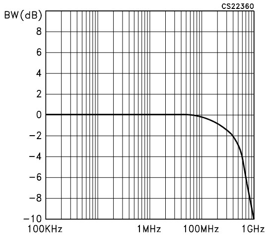
Figure 3: Bandwidth
