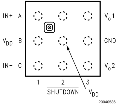
9 Bump micro SMD Package GAIN SELECT
