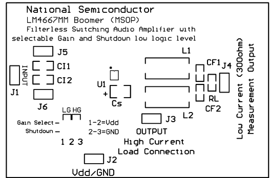
Silk Screen
