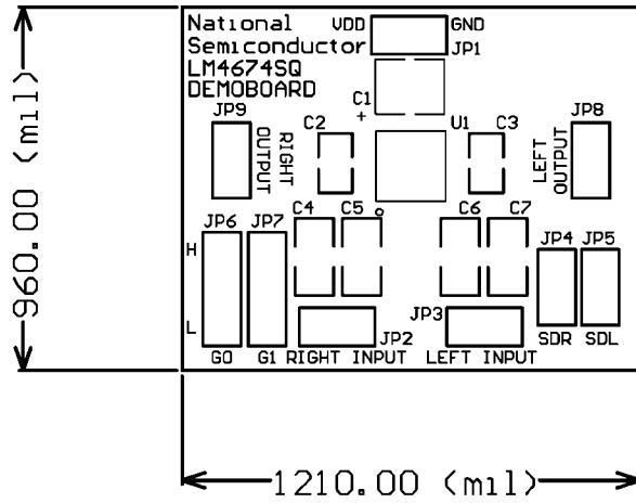
Top Silkscreen
