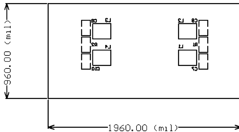
Bottom Silkscreen
