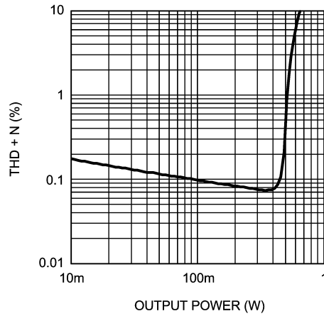
THD+N vs Output Power V_{DD} = 3.3V, R_L = 8\Omega, f = 1kHz Mode 5, BTL
