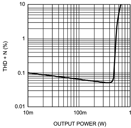
THD+N vs Output Power V_{DD} = 3.3V, R_L = 8\Omega, f = 1kHz Mode 1, BTL
