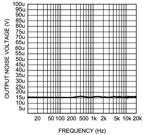
Noise Floor V DD = 1.5V, BTL Output 8Ω, 80kHz Bandwidth
