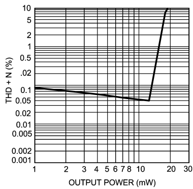
THD+N vs Output Power V_{DD} = 1.5V, R_L = 16\Omega, f = 1kHz Single Ended Output, A_V = -1
