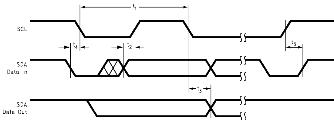
FIGURE 1. Serial Bus Timing Diagram
