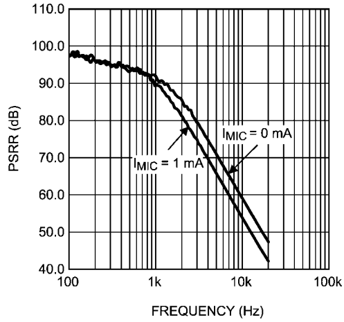
PSRR vs Frequency, Microphone Bias Mic1+ Mic2 AC shorted
