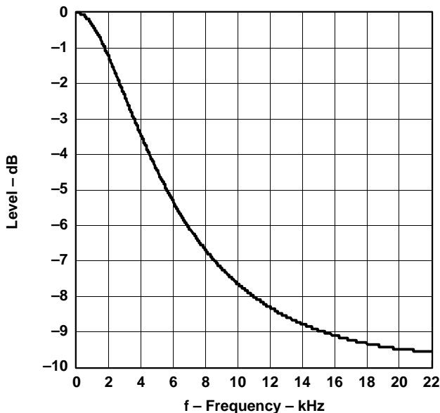
Figure 16. De-Emphasis ( f_S = 48 kHz)
