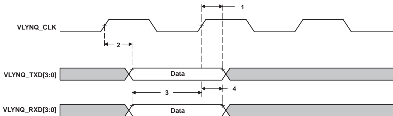
Figure 6-74. VLYNQ Transmit/Receive Timing
