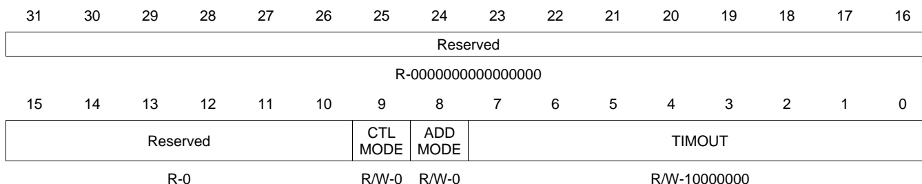
Figure 6-52. HPI_CTL Register
