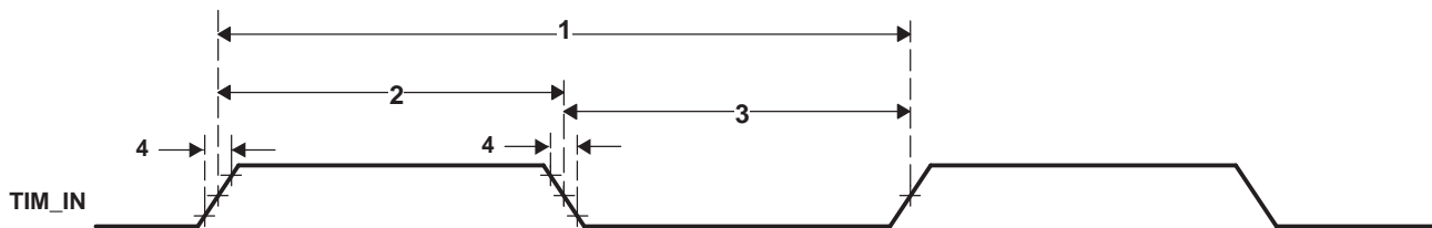
Figure 6-71. Timer Timing
