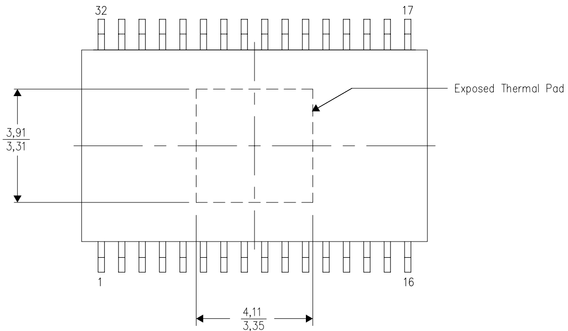
Top View Exposed Thermal Pad Dimensions
