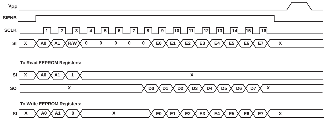
Figure 19. Serial Protocol
