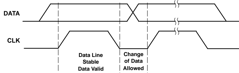
Figure 37. Bit Transfer on the Serial Interface
