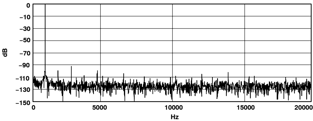
Figure 12. DAC FFT Plot ( T_A = 25^\circ\text{C} , 48 kpsps, -1 dB, 1 kHz Input, AVDD = DRVDD = 3.3 V, DVDD = 1.8 V, R_L = 16\ \Omega )
