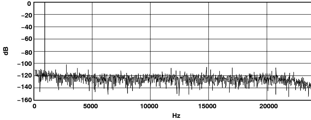
Figure 11. DAC FFT Plot ( T_A = 25^\circ\text{C} , 48 kpsps, 0 dB, 1 kHz Input, AVDD = 3.3 V, R_L = 10\ \text{k}\Omega )
