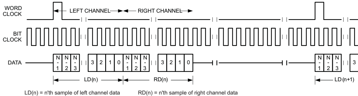
Figure 5-69. Timing Diagram for DSP Mode
