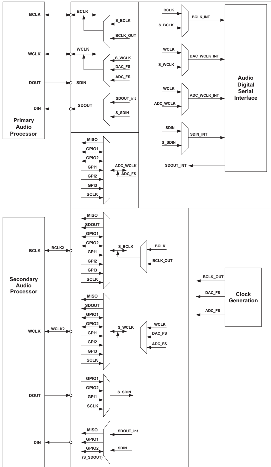
Figure 5-72. Audio Serial Interface Multiplexing
