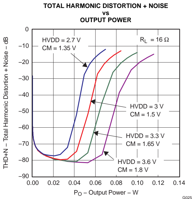
Figure 4-8. Headphone Output Power ( R_L = 16 \Omega )
