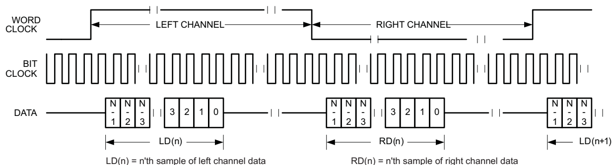
Figure 5-63. Timing Diagram for Left-Justified Mode with Offset=1
