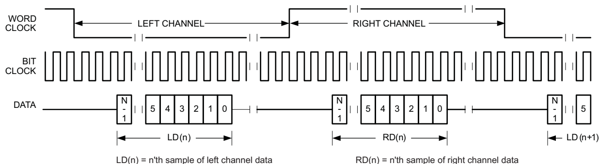
Figure 5-66. Timing Diagram for I 2 S Mode with offset=2
