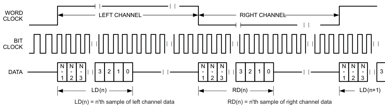
Figure 5-64. Timing Diagram for Left-Justified Mode with Offset=0 and inverted bit clock
