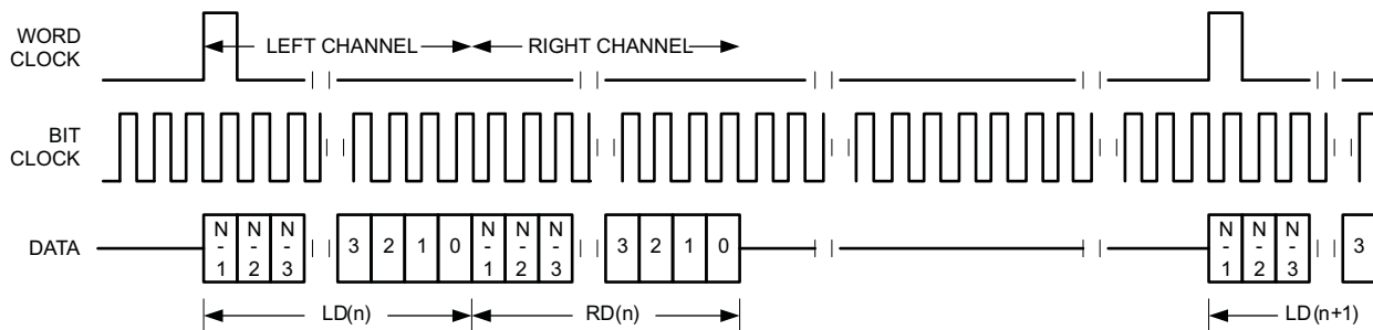
Figure 5-71. Timing Diagram for DSP Mode With Offset = 0 and Bit Clock Inverted
