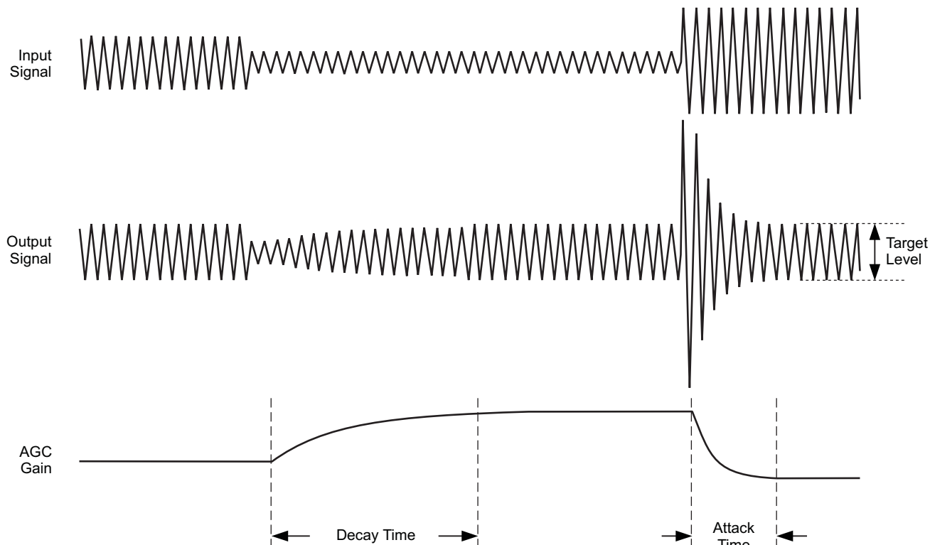
Figure 5-2. AGC Characteristics
