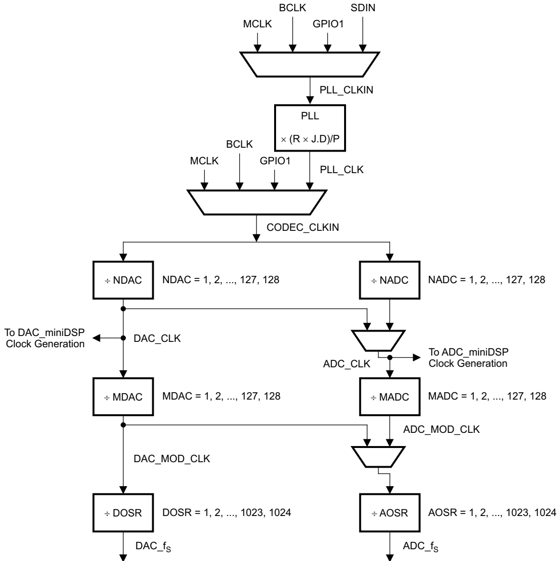
Figure 5-58. Clock Distribution Tree
