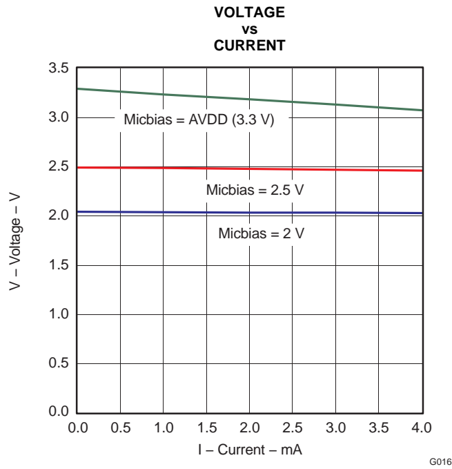
Figure 4-13. Micbias
