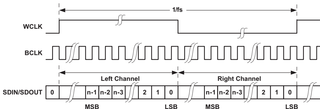
Figure 5-61. Timing Diagram for Right-Justified Mode
