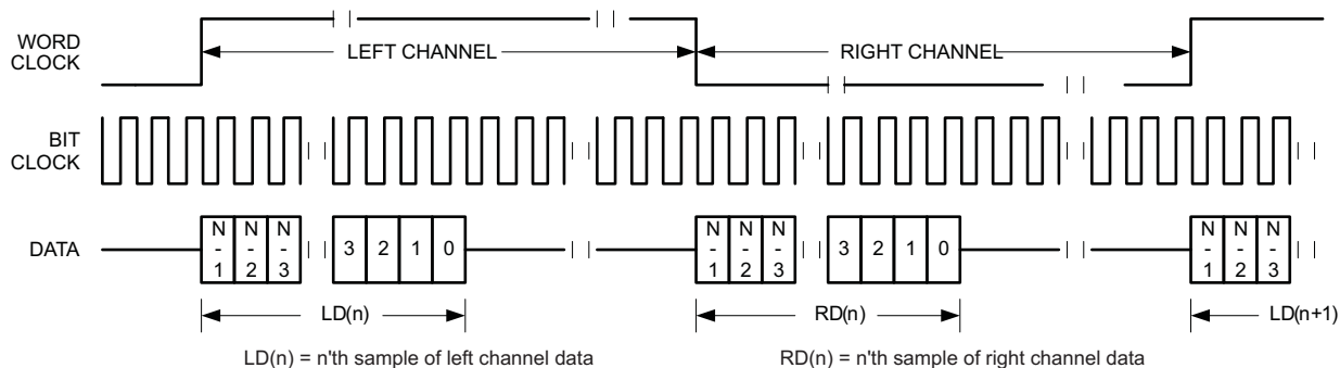
Figure 5-62. Timing Diagram for Left-Justified Mode
