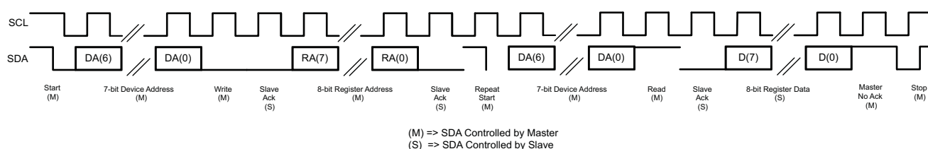
Figure 5-74. I 2 C Read
