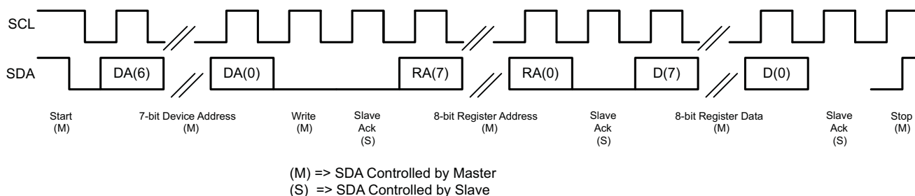
Figure 5-73. I 2 C Write
