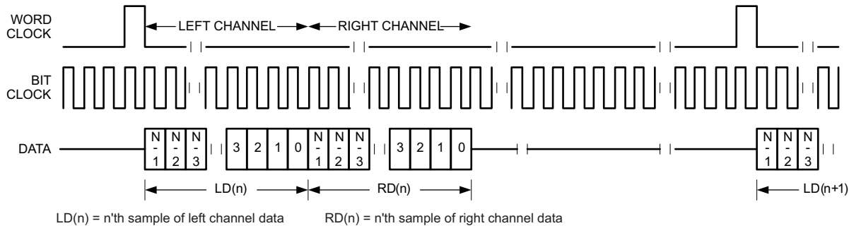
Figure 5-70. Timing Diagram for DSP Mode With Offset = 1
