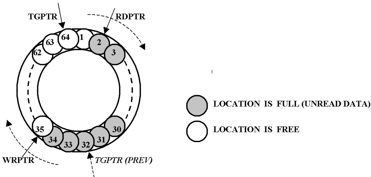
Figure 5-46. Circular Buffer
