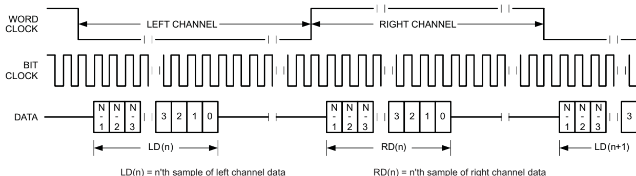
Figure 5-67. Timing Diagram for I 2 S Mode with offset=0 and bit clock invert
