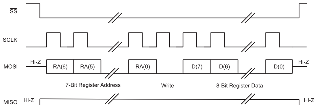
Figure 5-75. SPI Timing Diagram for Register Write
