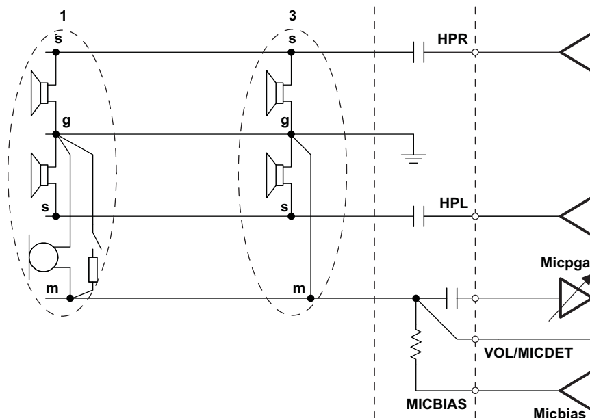
Figure 5-34. Jack Connections for Headset Detection
