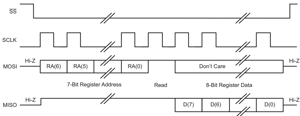
Figure 5-76. SPI Timing Diagram for Register Read
