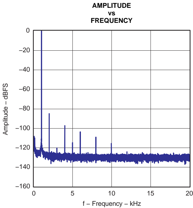
Figure 4-6. FFT - DAC to Line Output
