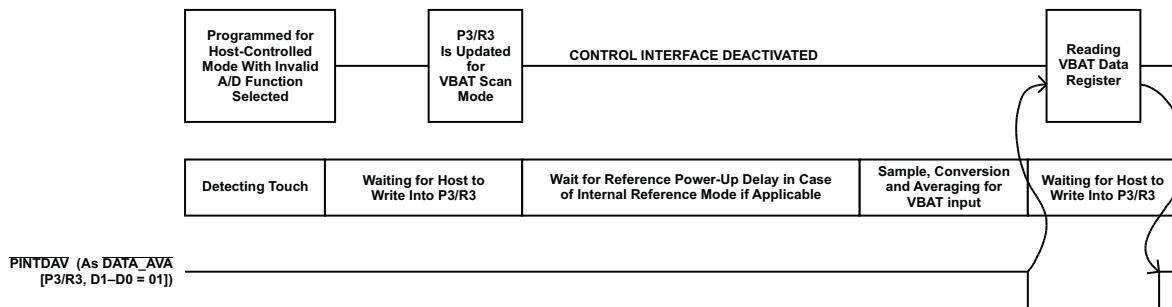
Figure 5-55. Host-Controlled BAT1 Scan Mode
