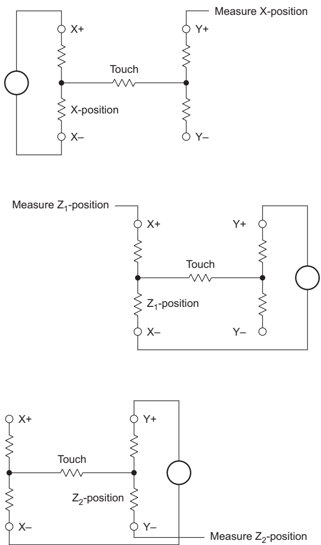
Figure 5-38. Pressure Measurement
