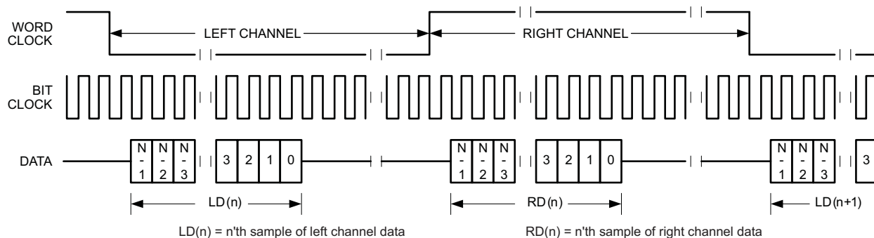
Figure 5-65. Timing Diagram for I 2 S Mode
