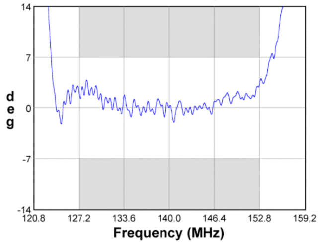
Phase Linearity
