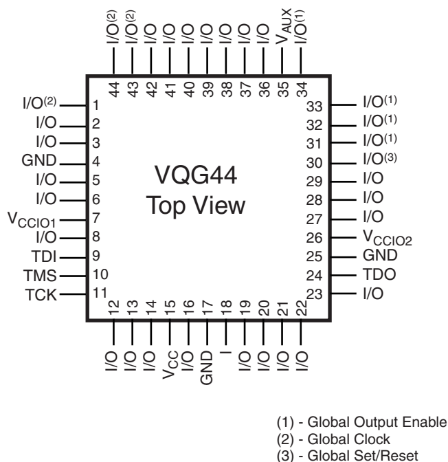
Figure 6: VQG44 Package
