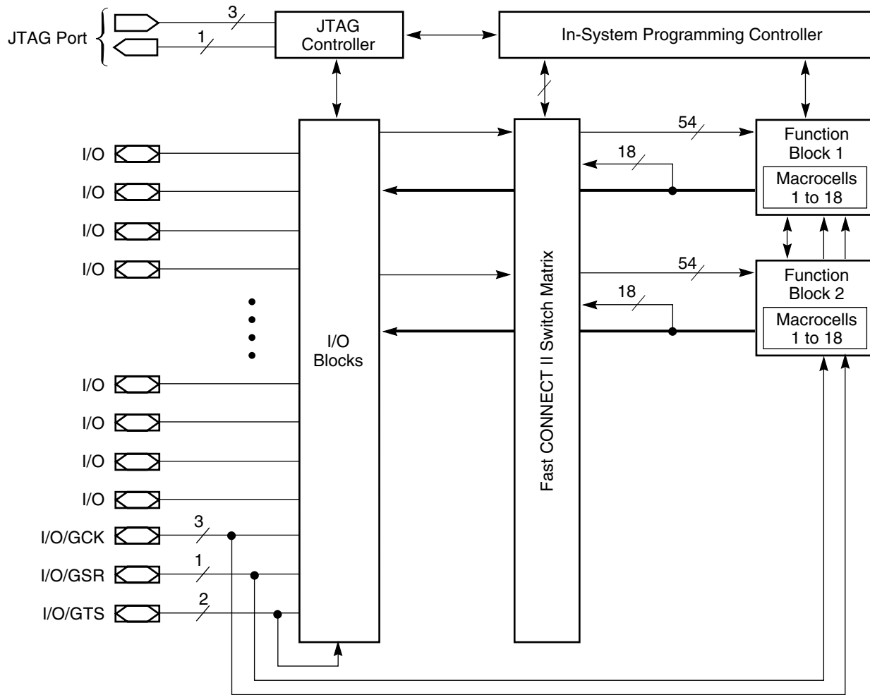
Figure 2: XA9536XL Architecture
