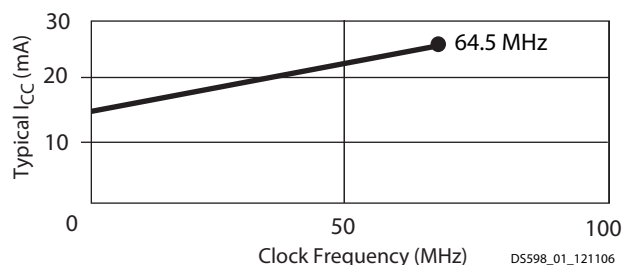
Figure 1: Typical I_{CC} vs. Frequency for XA9536XL
