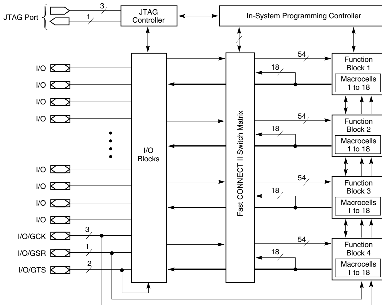
Figure 2: XA9572XL Architecture
