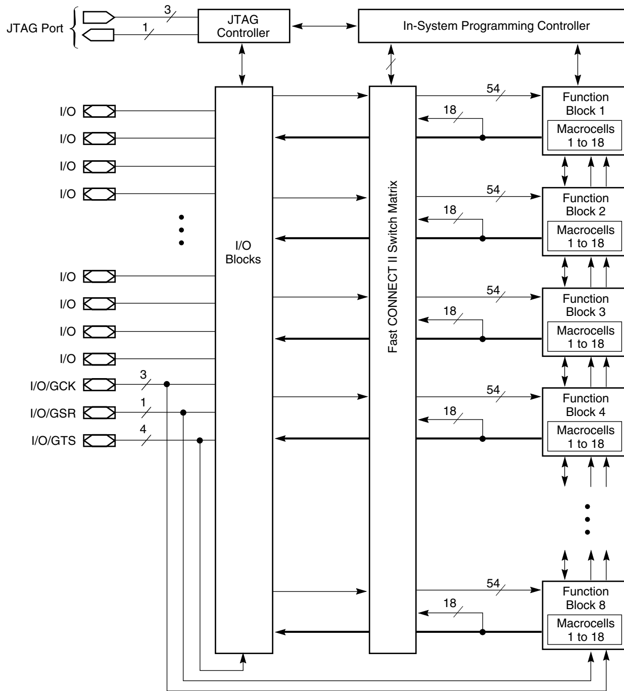
Figure 2: XA95144XL Architecture
