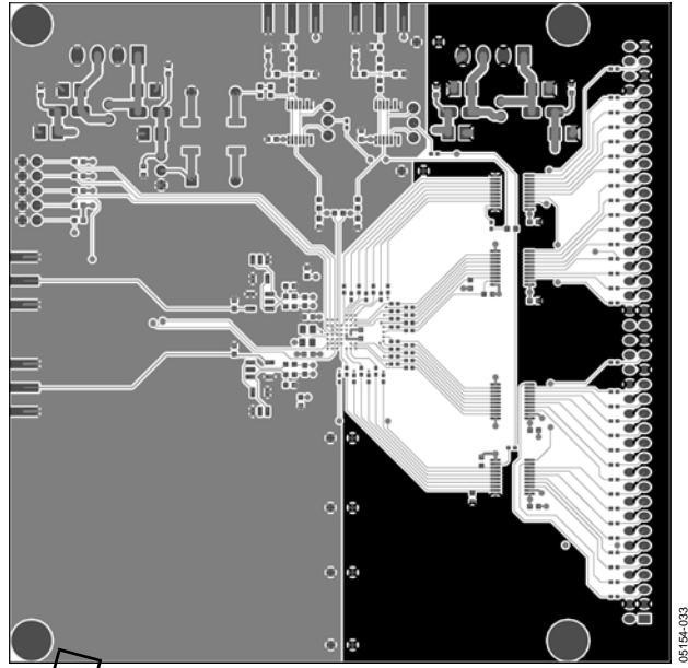
Figure 27. AD15252 Evaluation Board Bottom Signal
