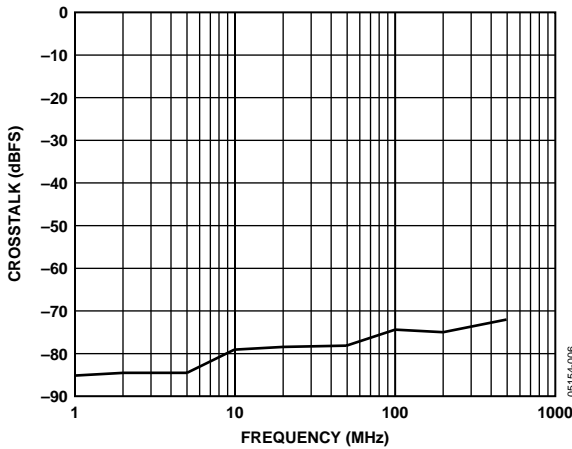
Figure 5. Typical Crosstalk
