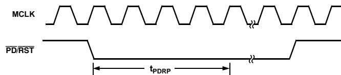
Figure 25. Power-Down/Reset Timing
