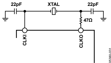
Figure 25. Crystal Connection
