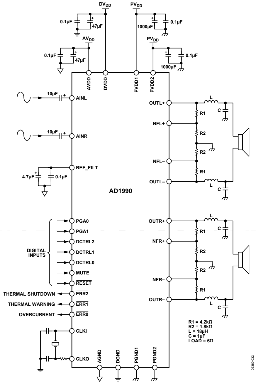
Figure 26. Typical Application Circuit
