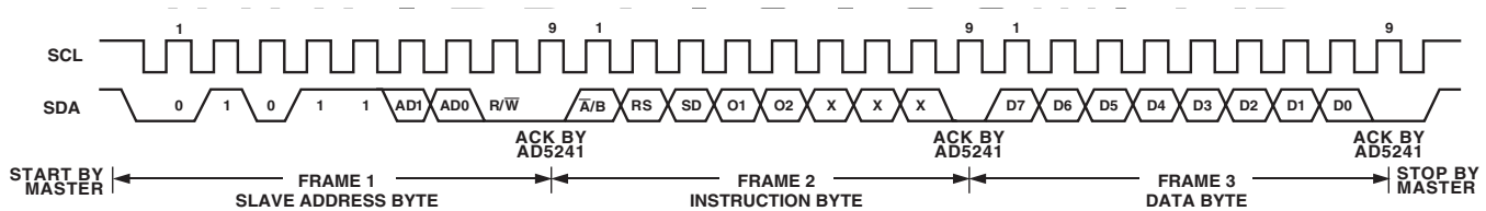
Figure 2. Writing to the RDAC Serial Register
