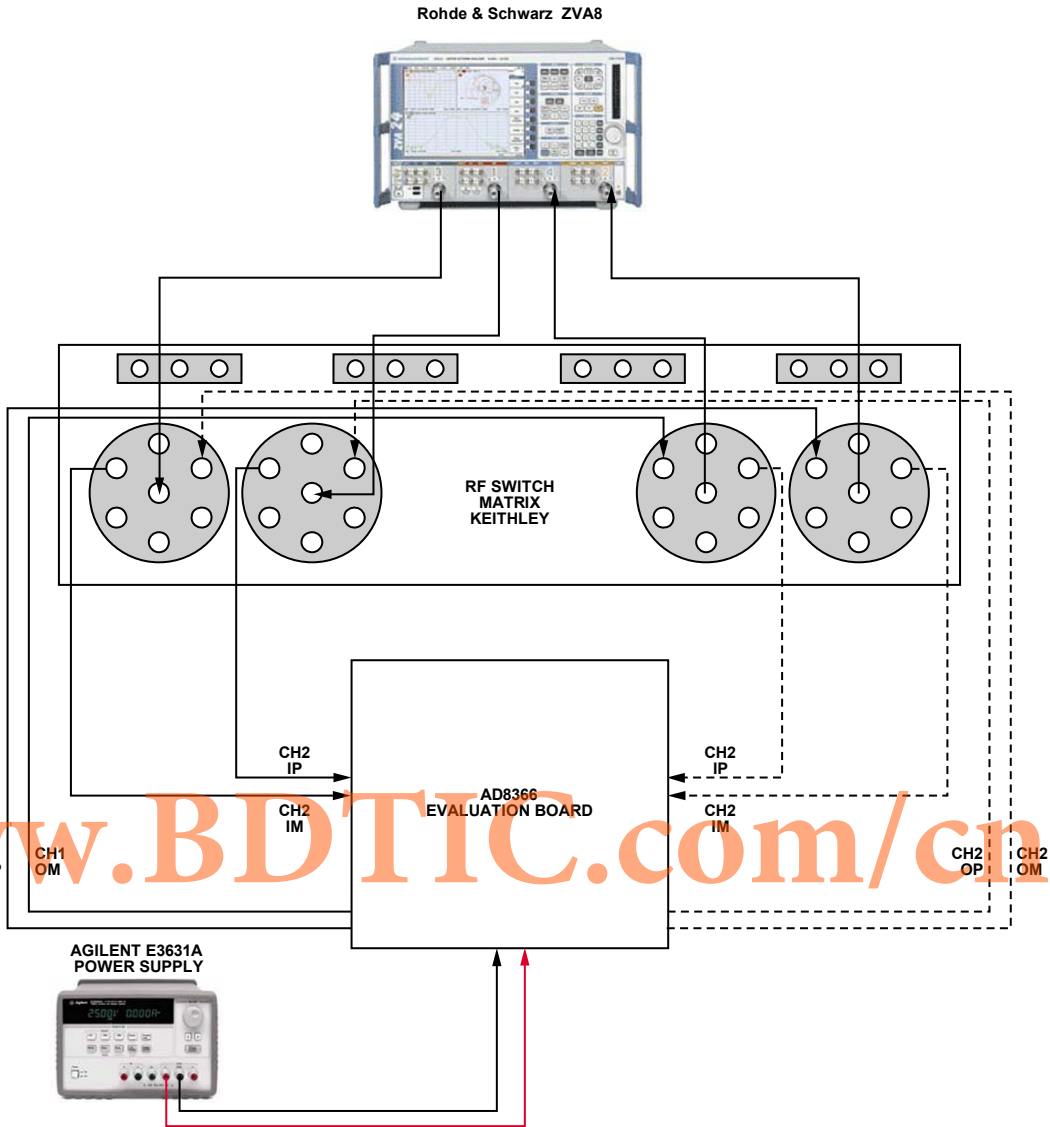
Figure 59. Characterization Setup, Differential Measurements
