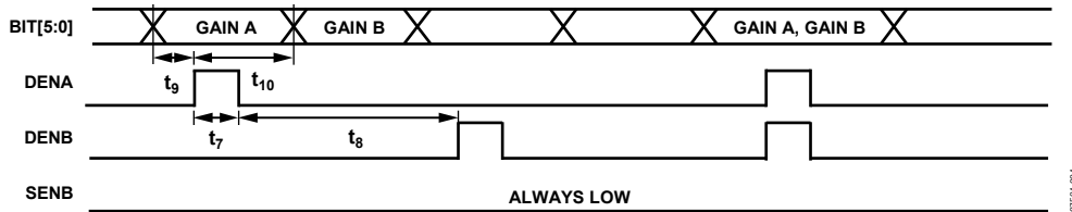
Figure 3. Parallel Port Timing Diagram
