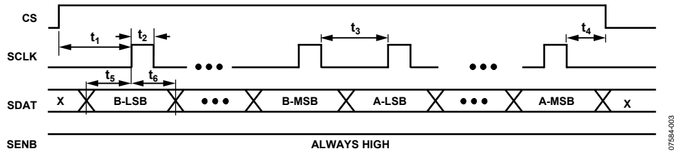
Figure 2. SPI Port Timing Diagram
