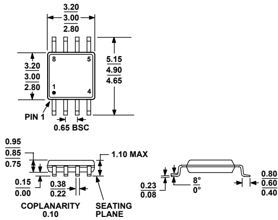
Figure 27. 8-Lead Mini Outline Package [MSOP] (RM-8)
