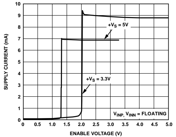
Figure 20. Supply Current vs. Enable Voltage
