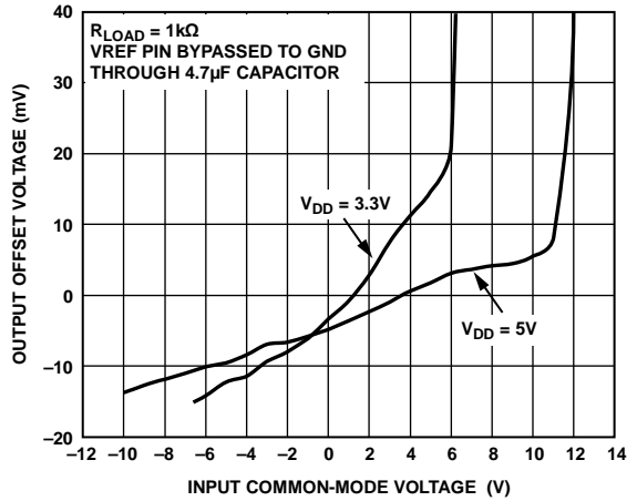
Figure 19. Output Offset Voltage: V_{OUT} - V_{REF}
