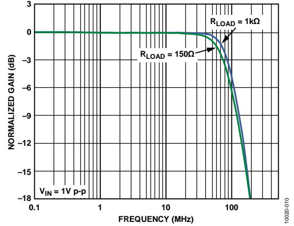
Figure 7. Large Signal Frequency Response vs. Load
