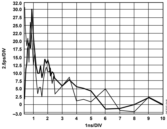
Figure 15. Comparator t_{PD} vs. Pulse Width
