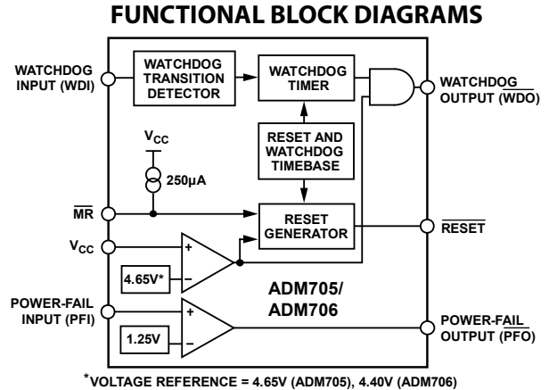
Figure 1. ADM705/ADM706
