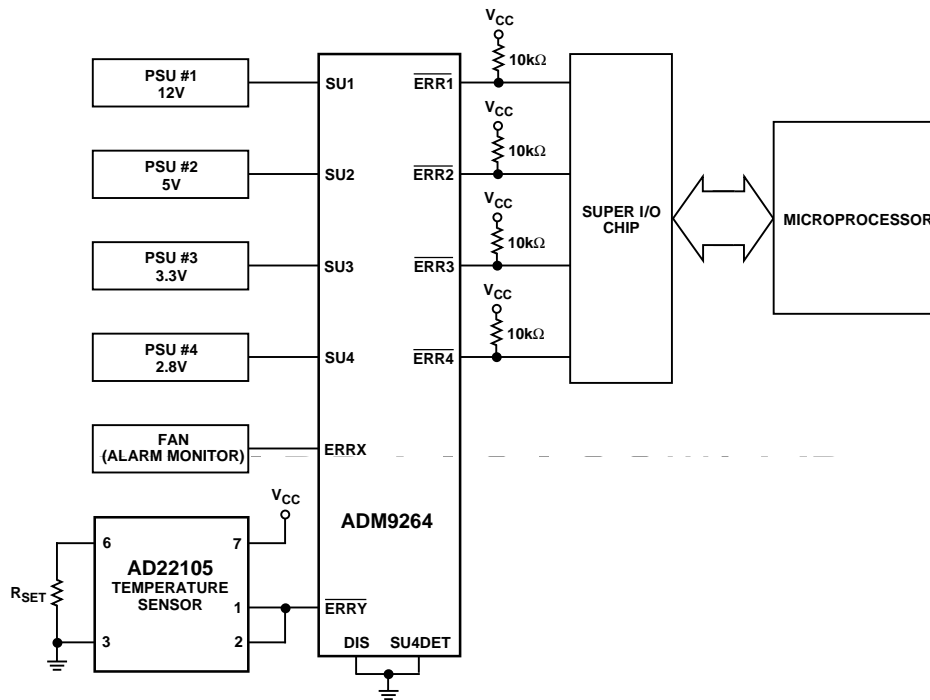
Figure 23. Typical Application of ADM9264
