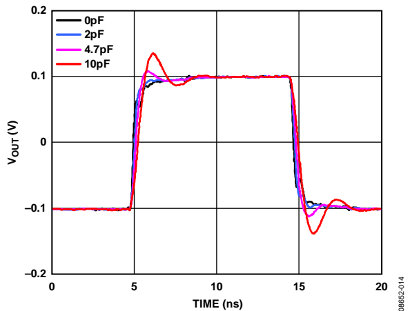
Figure 8. ADV3221 Small Signal Pulse Response vs. Capacitive Load, 200 mV p-p
