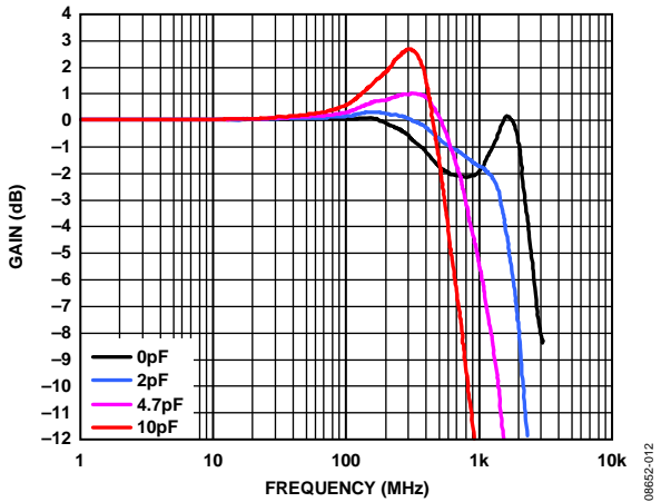
Figure 6. ADV3221 Small Signal Response vs. Capacitive Load, 200 mV p-p
