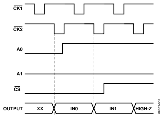
Figure 3. Programming Example
