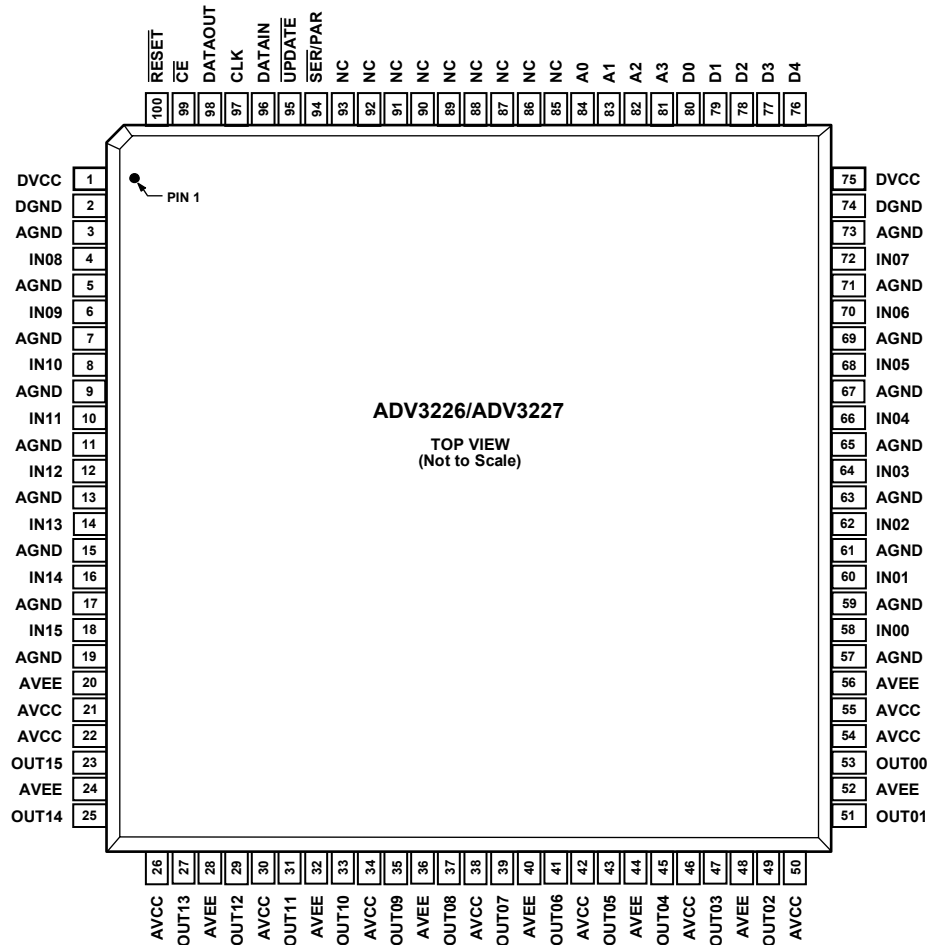
Figure 5. Pin Configuration
