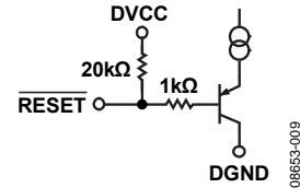
Figure 63. Reset Input
